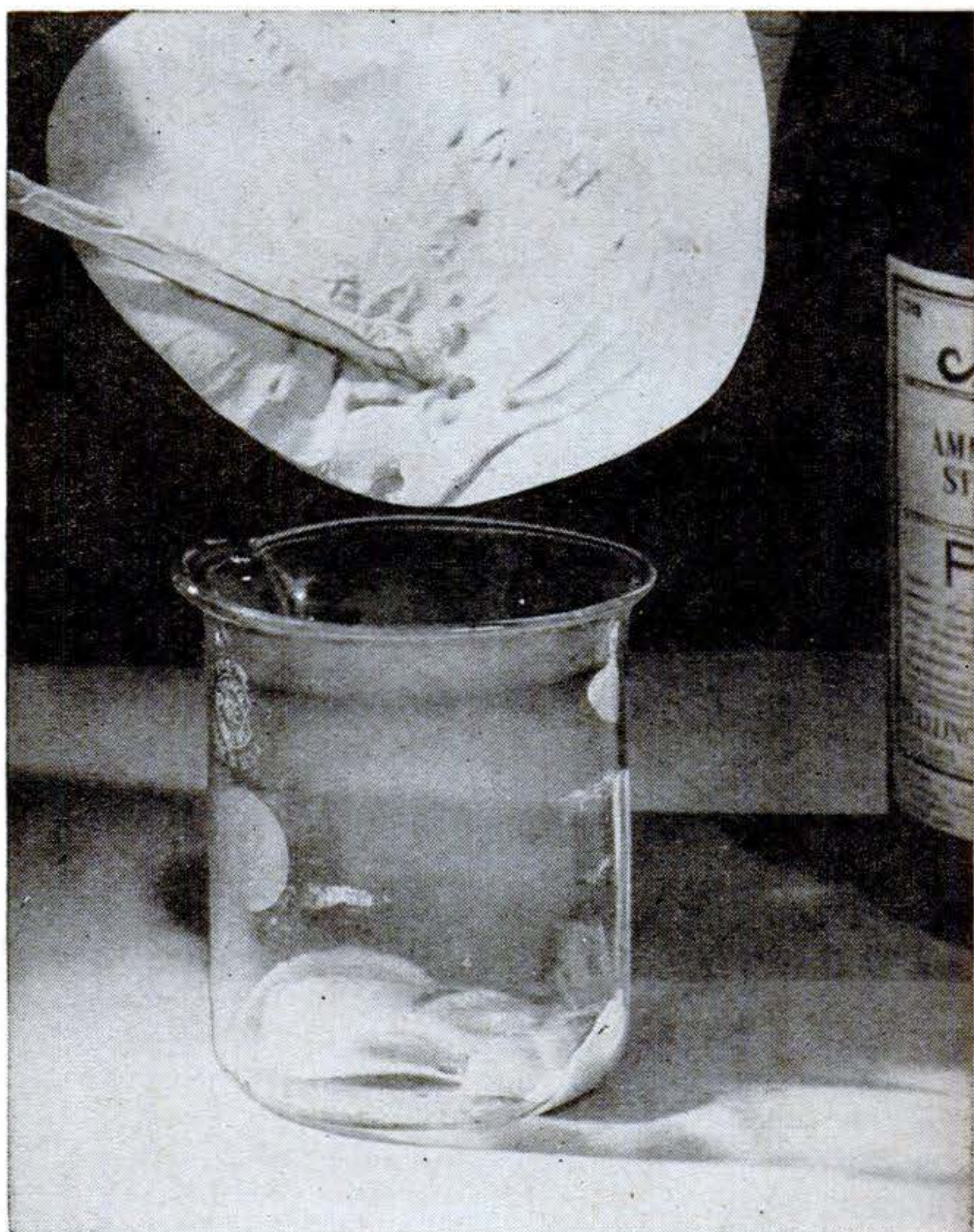
Copper hydroxide precipitates as a pale blue compound. Wash and filter this. Then dissolve in just a little strong ammonium hydroxide.
